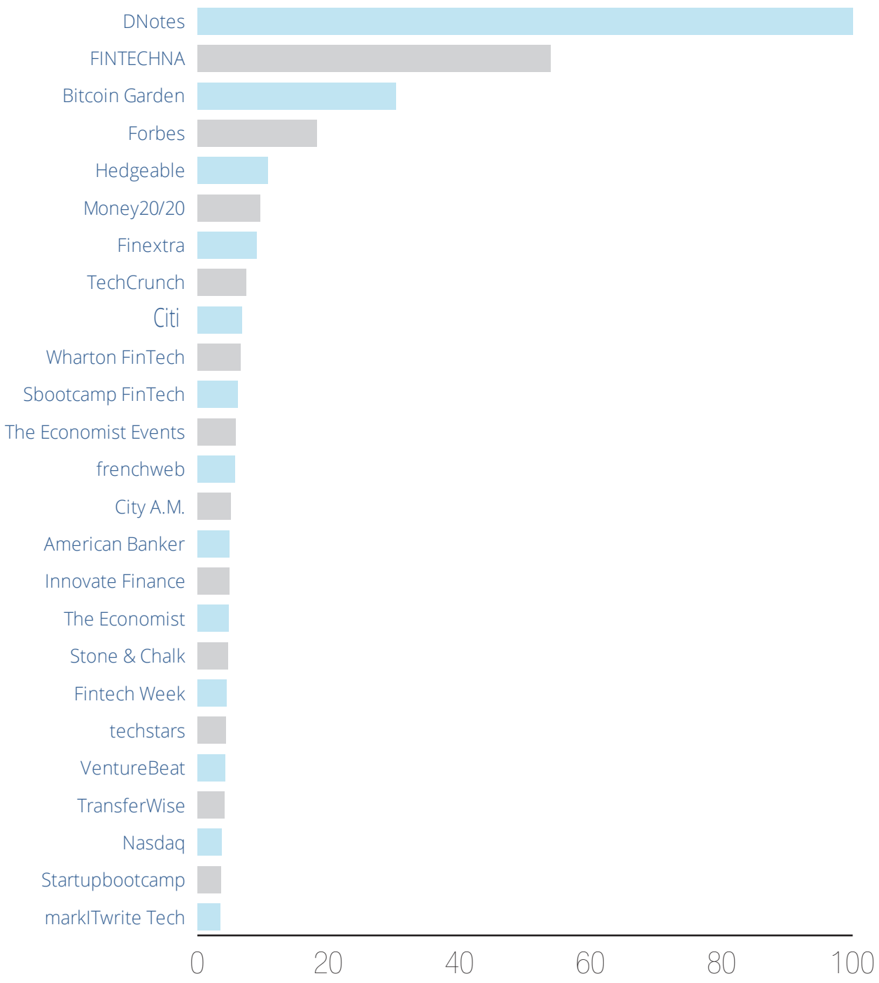
Normalised PageRank
